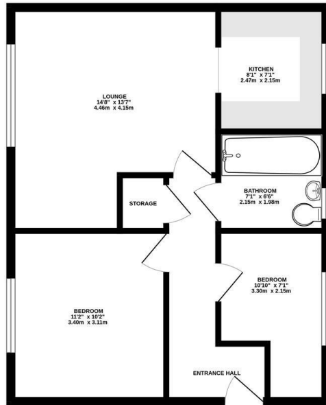
FIRST FLOOR 533 sq.ft. (49.5 sq.m.) approx.
